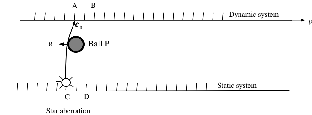
Figure 17 Relativity thinks that when light appears at \Delta t = \frac{CA}{c_0} , because ball P is in the \overline{CA} line, so it thinks that light has to rotates ball P and takes more steps, which means space is curving. (In order to strike the eye, it overstates dynamic system speed)
