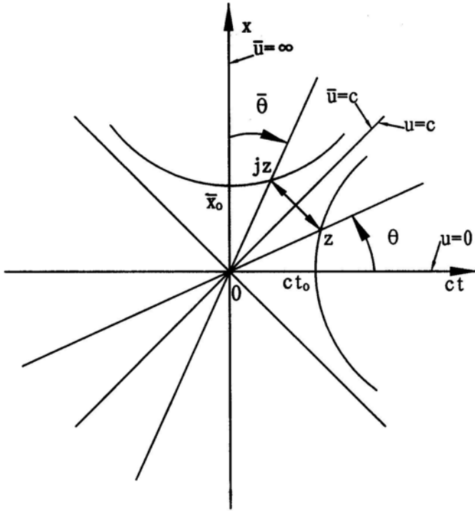
Fig. 1. Mathematical theory of space-time with SASC
