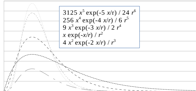
Illustration 2: Exponential distributions
