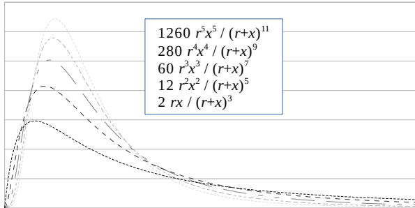
Illustration 1 : Polynomial distributions
