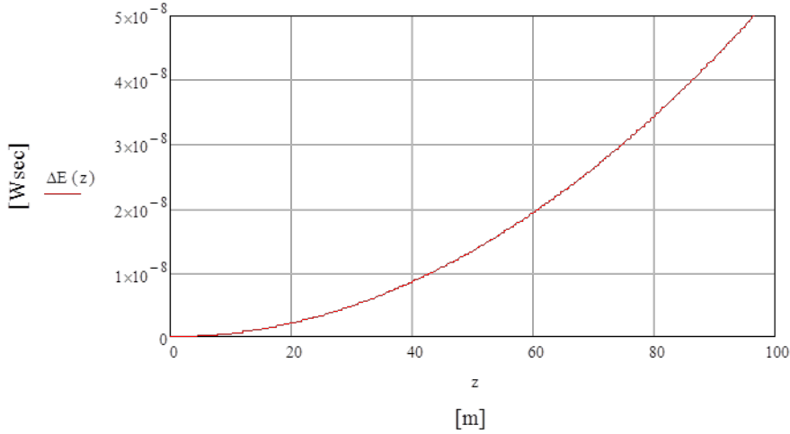
FIG.1 the dependency of energy loss due to radiation for a 10,000kg uniformly accelerated test body in a flat space-time simulating the free fall in a gravitational field of Earth on the travelled distance z.
